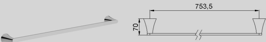
FR164.02/K4 Barral 760 mm. CR - BB - BG - BK - BN PB - PG - PN - SGR
